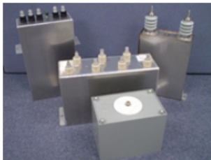
Welded Air Cooled
